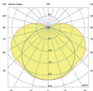
Titan Delta Code: 6418 1400
